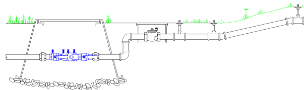
Double Check Valve Assembly in Below-Ground Box
