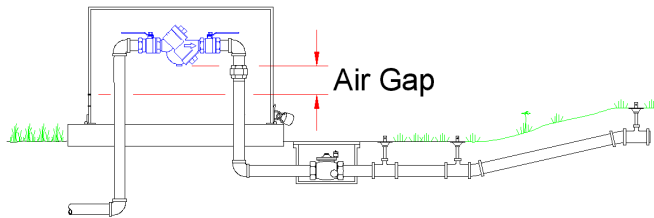
Reduced Pressure backflow Assembly in Above-Ground Enclosure
